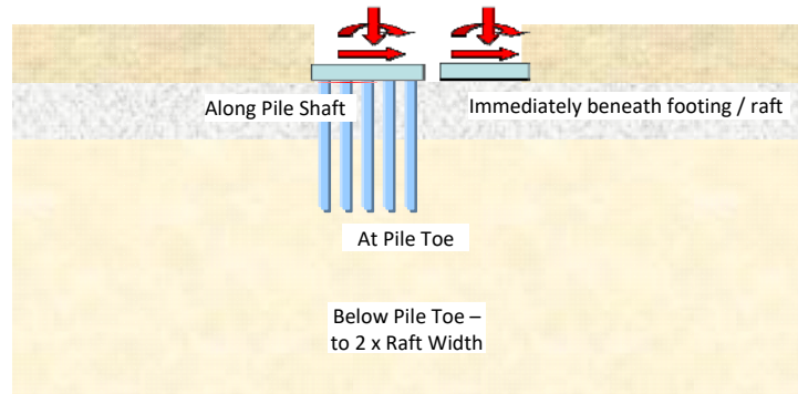
Fig. 4. Design considerations for raft and piled-raft
