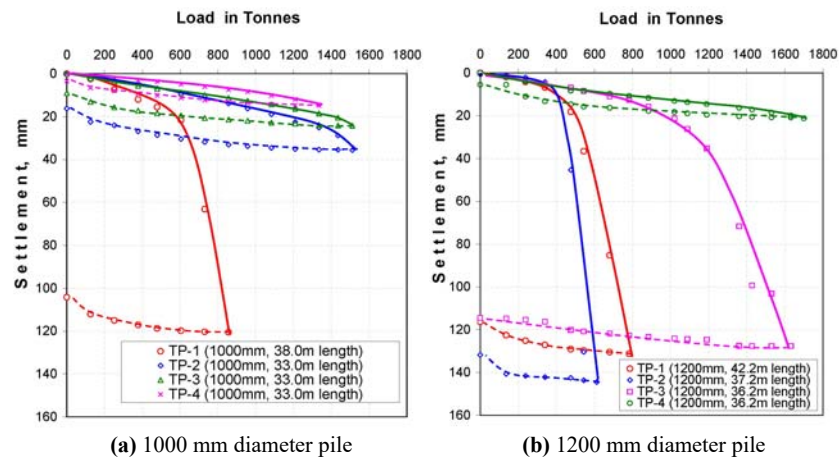
Fig. 7 Results of pile load tests
