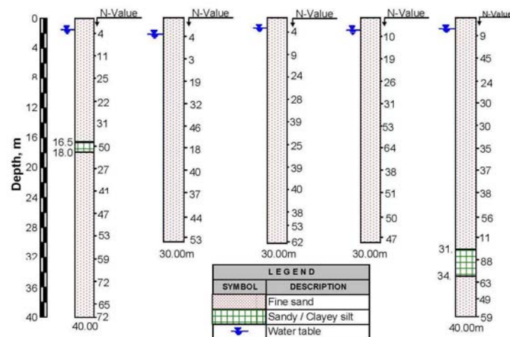
Fig. 5. Typical Profiles of boreholes drilled for initial investigation
