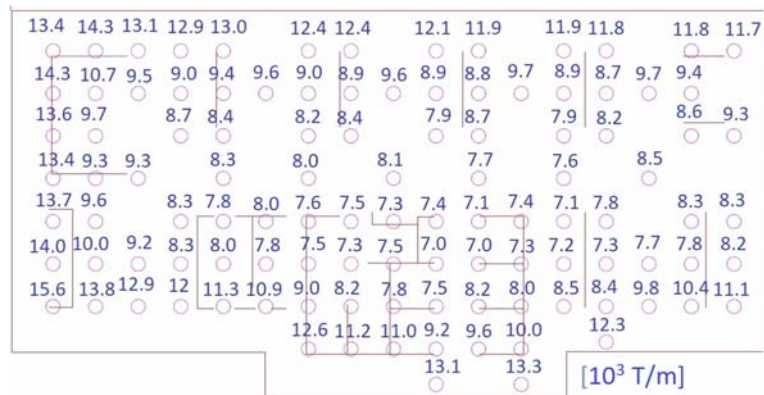
Fig. 16. Pile spring constant
