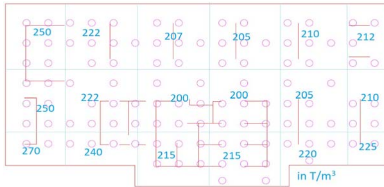
Fig. 15. Soil spring constant
