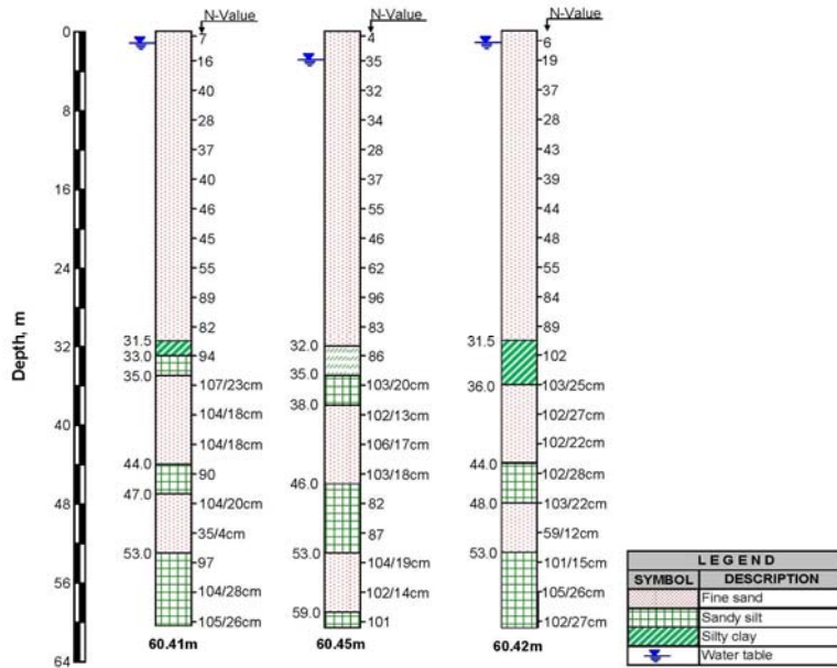
Fig 9. Data from deep boreholes drilled for piled-raft analysis
