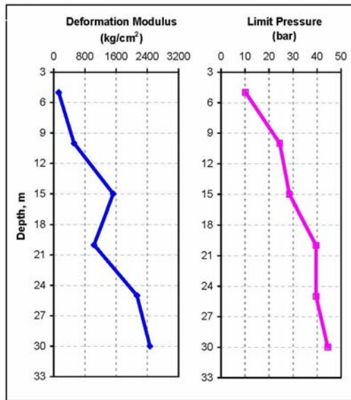
Fig. 10. Pressuremeter modulus and limit pressure versus depth – Typical results from one borehole
