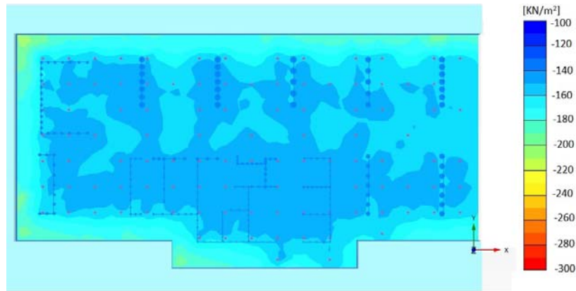
Fig. 14. Pressure Contours at soil-raft interface
