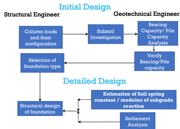
Fig 1. Flow chart explaining the role of structural engineer and geotechnical engineer
