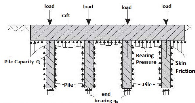
Fig. 3. Load transfer mechanism in piled raft
