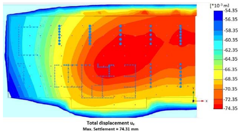
Fig. 13. Settlement Contours
