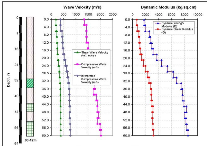
Fig. 11. Wave velocities and dynamic moduli from cross-hole seismic test
